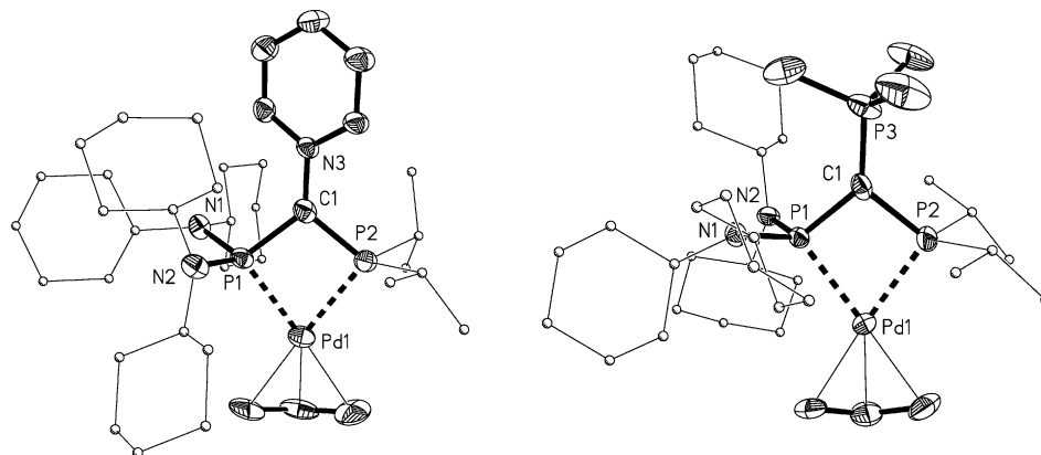
Figure 4. Thermal ellipsoid diagrams (50% probability) of 7b (left) and 8b (right). For clarity, the cyclohexyl and isopropyl groups are simplified. Only one position is shown for the disordered isopropyl groups at phosphorus and meso carbon atoms of the allyl group. The tetraphenylborate anion has been omitted. Selected bond lengths (Å) and angles (°): 7b , P1–C1 1.769(5), P2–C1 1.776(6), C1–N3 1.424(7), P1–Pd1 2.2969(15), P2–Pd1 2.2862(15), P1–C1–P2 102.0(3), P1–C1–N3 129.8(4), P2–C1–N3 128.2(4), P1–Pd1–P2 73.89(5); 8b , P1–C1 1.764(3), P2–C1 1.771(3), C1–P3 1.741(3), P1–Pd1 2.3142(9), P2–Pd1 2.2845(10), P1–C1–P2 99.01(16), P1–C1–P3 133.41(18), P2–C1–P3 127.58(18), P1–Pd1–P2 71.55(3).
