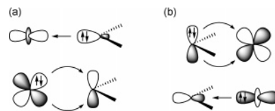
Figure 7. Schematic representations of the MC interactions involved in Fischer-type carbene complexes (a) and in metalladiphosphinocarbenes (b).
