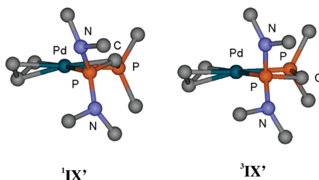
Figure 5. Optimized structures for singlet and triplet metalladiphosphanycarbenes IX' (hydrogen atoms have been omitted for clarity).
