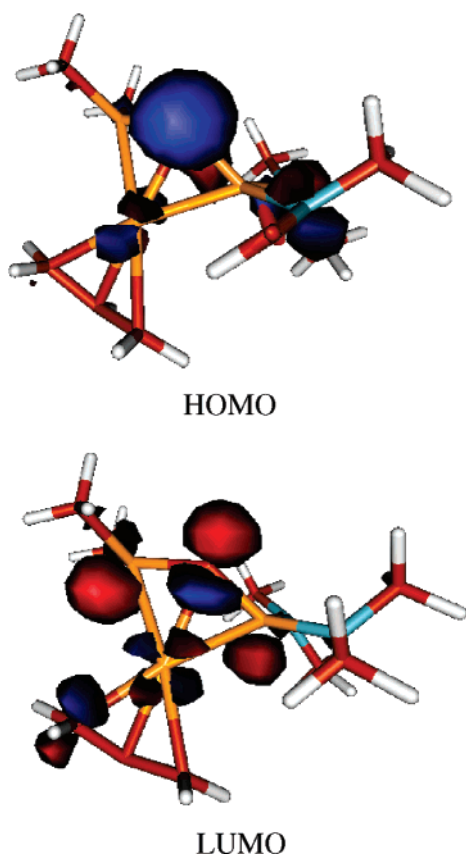
Figure 6. Plots of the frontier orbitals for ^1\text{IX}' .
