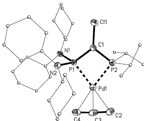
Figure 3. Thermal ellipsoid diagram (50% probability) of 3b . For clarity, the cyclohexyl and isopropyl groups are simplified and only one position of the disordered meso carbon atoms of the allyl group is shown. Selected bond lengths (Å) and angles (°): P1–C1 1.727(3), P2–C1 1.733(3), C1–Cl1 1.778(3), P1–Pd1 2.3160(7), P2–Pd1 2.2886(7), Pd1–C2 2.216(3), Pd1–C3 2.164(4), Pd1–C4 2.218(3), C2–C3 1.366(5), C3–C4 1.384(5), P1–C1–P2 103.80(14), P1–C1–Cl1 130.18(16), P2–C1–Cl1 125.91(15), P1–Pd1–P2 72.49(2).
